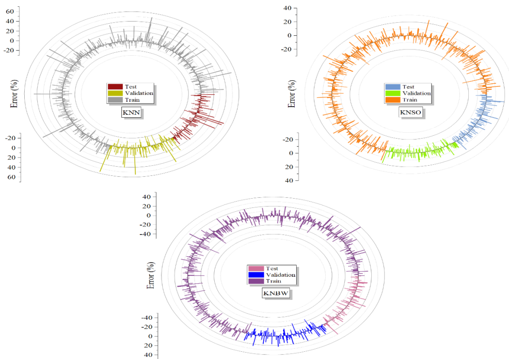
Fig. 3. The models' error percentage based on the Radial Stacked Bar plot.
