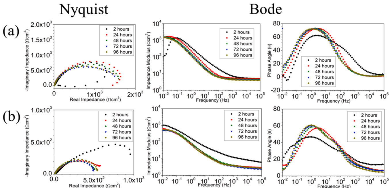
Fig. 10. EIS of the as-received (a) and laser hardened (2 mm, 1 mm/s, 153.3 W and 25 % overlapping) (b) samples in 0.6 M NaCl.
